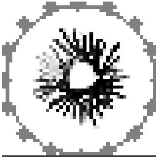
Figure 2: Pixelated reflection-mode ultrasound tomogram of a hydrocyclone.
