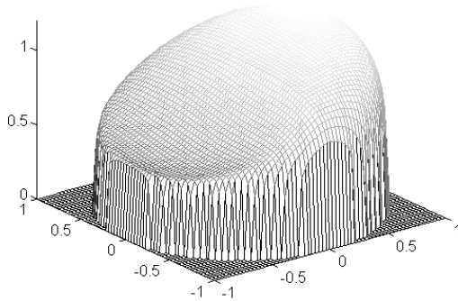
Figure 5. 3-D mesh of the velocity profile after the bend
