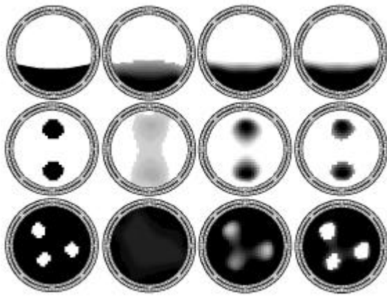
Figure 2 Visual evaluation of the reconstructed tomograms when using LBP thresholded, SIRT weighted, SIRT weighted and thresholded relative to the test reference for synthetic stratified, slug and bubble flows.
