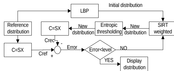
Figure 1 A schematic diagram for the SIRT weighted and thresholded
