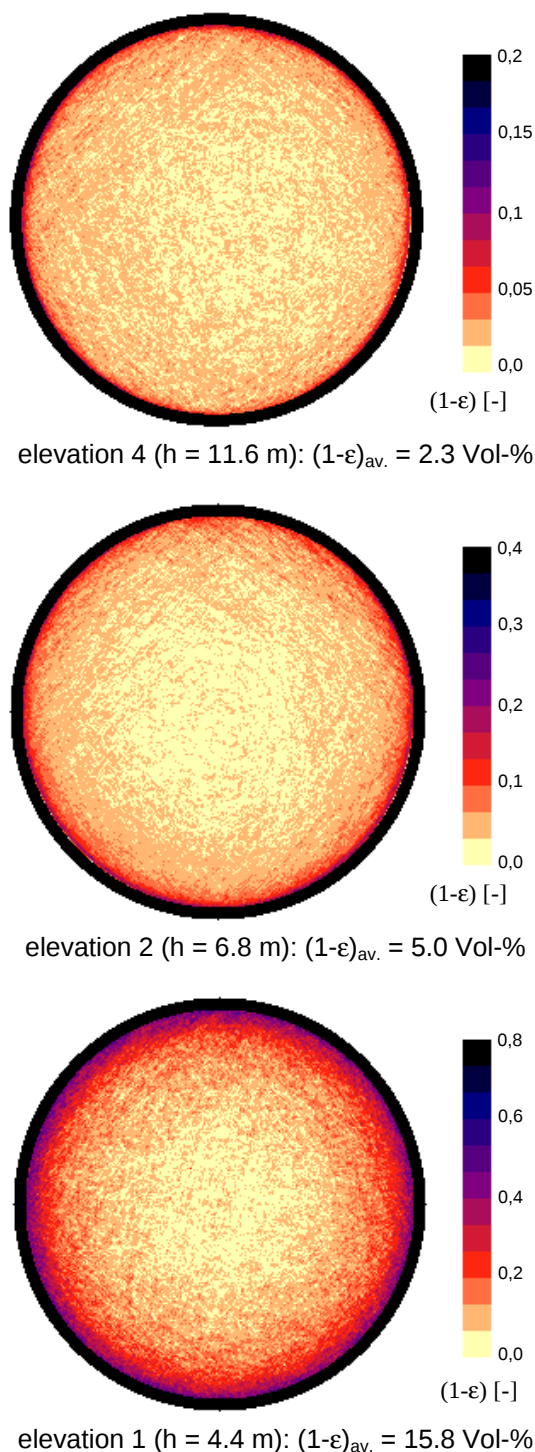
Figure 9: Solids concentration distribution in the riser ( U_G = 2.7 \text{ m/s} , G_s = 195 \text{ kg}/(\text{m}^2\text{s}) )
