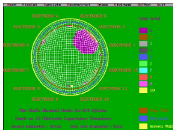
Figure 4b: Reconstructed Pos 1 image based on LBP algorithm
