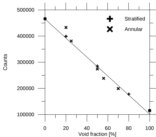
Figure 4. The measured number of counts in the full energy peak plotted against the void fraction with the detector located at 52° (the source is at 0°). The legends and the solid line represent the measured data and best curve fit, respectively [8].
