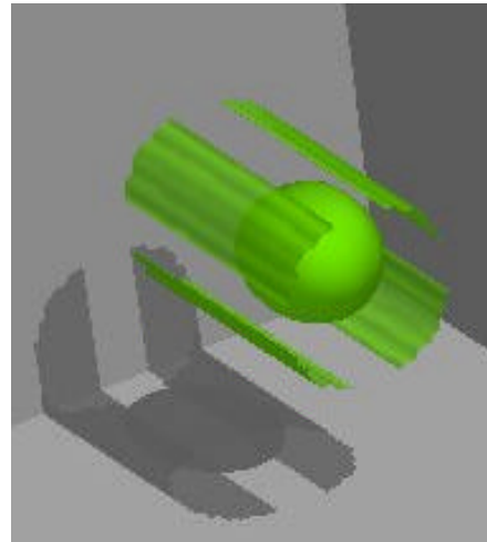
Figure 4 LBP images of ceramic spherical phantom presented as pseudo three-dimensional iso-contour plot.
