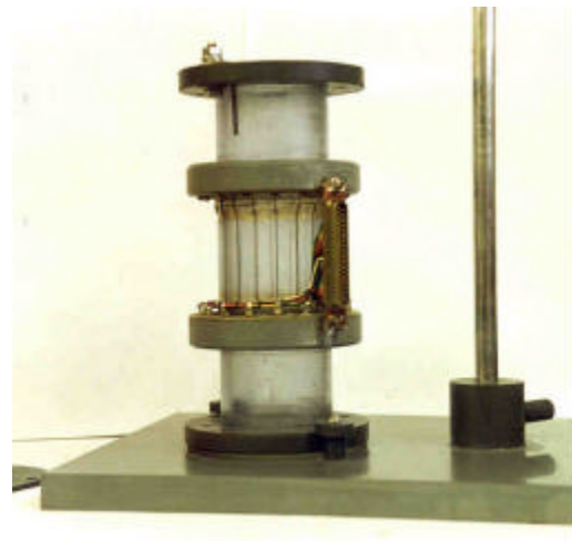
Figure 1 (a) Meso scale sensor with axially extended electrodes after [13]. (b) The macro scale sensor used in the rod and sphere phantom evaluation.
