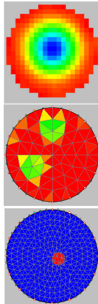
Figure 2 Images of single glass rod, dual glass rods and single steel rod reconstructed using (a) LBP, (b) MNR and (c) PM respectively.
