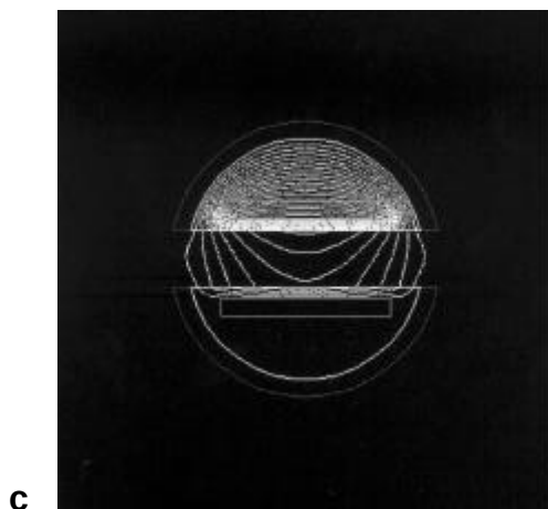
Figure 2. a) Cross-section of the probe, used as a starting point for numerical simulations; b) equipotential lines for the probe immersed in the medium of \epsilon=1 ; c) equipotential lines for the probe immersed in the medium of \epsilon=80
