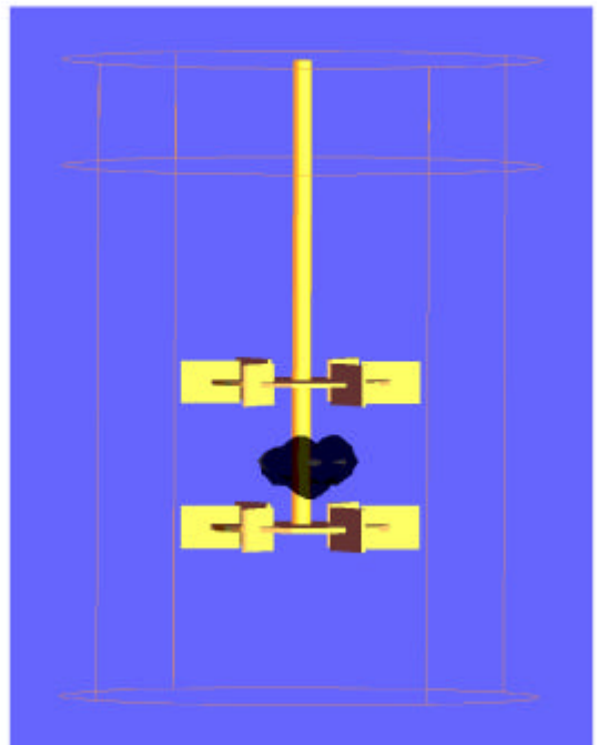
Figure 6: Mixing with the combination of the two Rushton turbines
