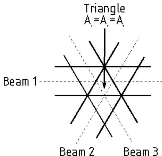
Figure 4: Tomographic reconstruction with different elements schemes.
