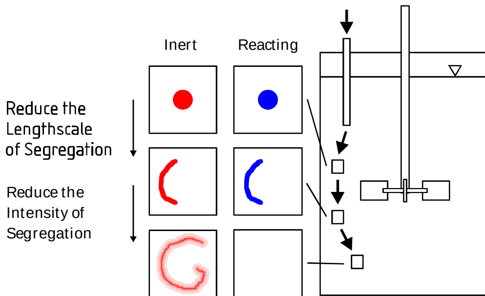
Figure 1: Course of the laminar mixing process and its influence on inert and reacting dyes.
