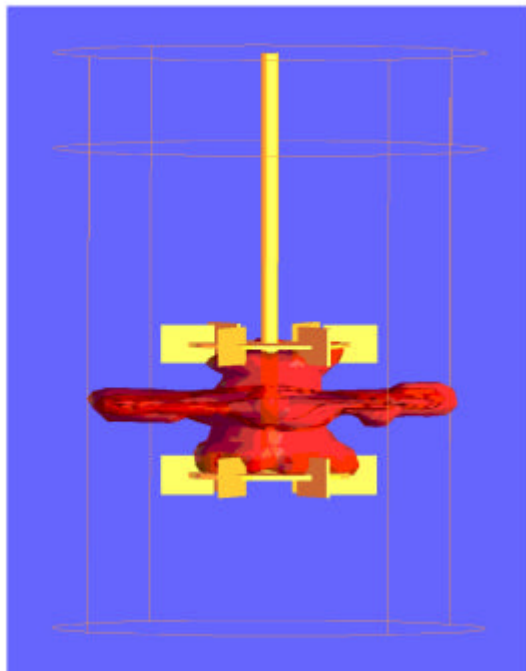
Figure 6: Mixing with the combination of the two Rushton turbines
