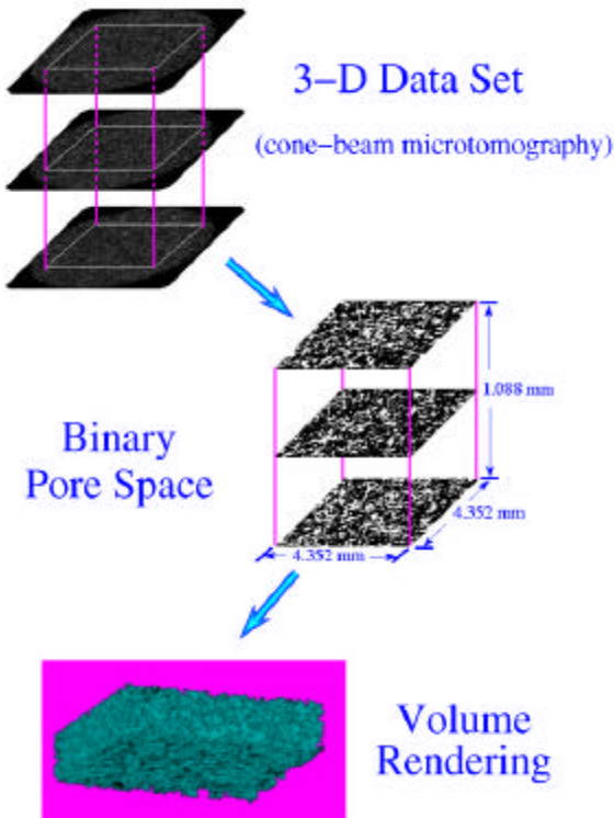
Figure 5: Schematic diagram for visualization of pore structure from original cone beam 3-D data.
