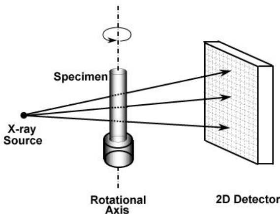
Figure 2: Schematic diagram of the cone-beam x-ray microtomography system.
