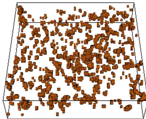
Figure 12: 3-D view of spatial distribution isolated pores after 2 stages of E/D.
