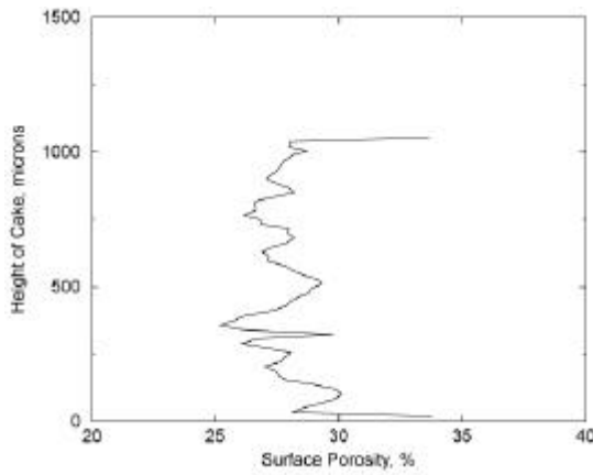
Figure 6: Surface porosity versus height of filter cake.
