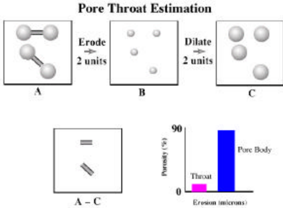
Figure 9: Schematic representation of estimation of pore body and throat using successive erosion/dilation stages.
