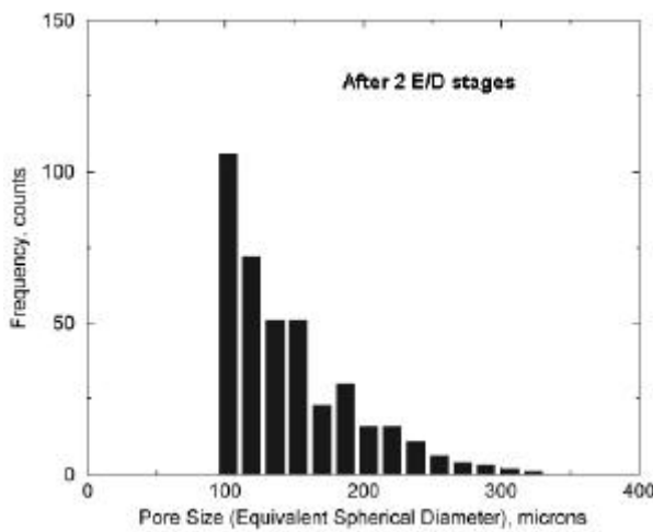
Figure 13: Pore size distribution after 2 stages of E/D.
