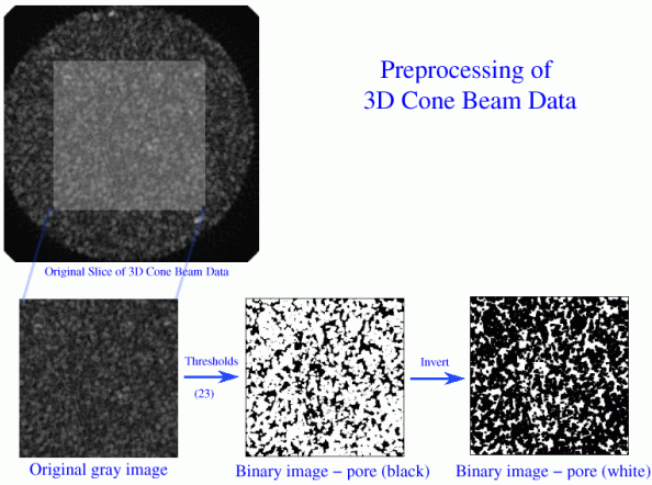
Figure 4: Pre-processing the cone beam data to extract pore features.
