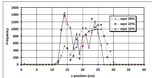
Figure 9: Axial position profiles for a series of experiments using wide particle size distribution polyethylene.
