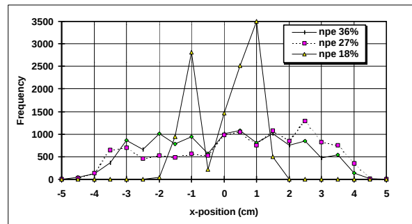
Figure 8: Horizontal position profiles for a series of experiments using narrow particle size distribution polyethylene.
