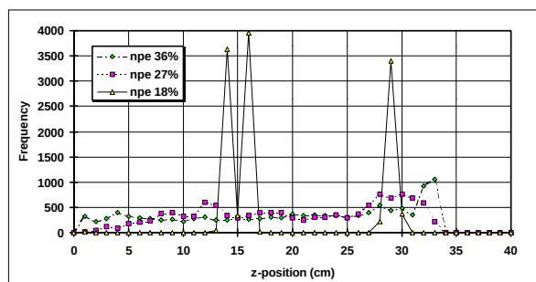
Figure 10: Axial position profiles for a series of experiments using narrow particle size distribution polyethylene.
