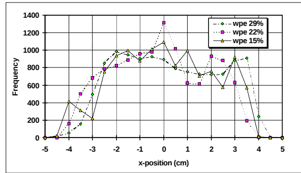
Figure 7: Horizontal position profiles for a series of experiments using wide particle size distribution polyethylene.
