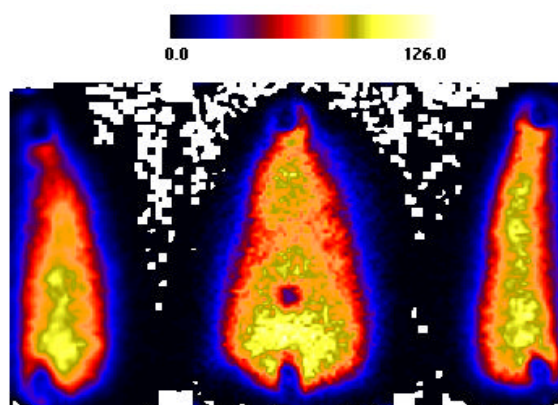
Figure 6: Gamma-camera imaging of the displacement of heavy oil by brine. Visualization of sweep efficiency.
