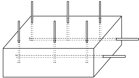
Figure 2: Schematic of the physical model used in the porous media displacement experiments
