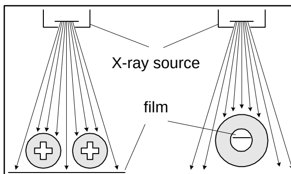
Figure 1: Radiographic test of the powder rod through one and two walls
