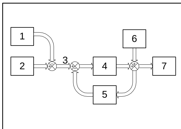
Figure 13: Differential tomography scheme
