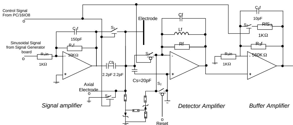
Figure 3 MPT drive/detect board
