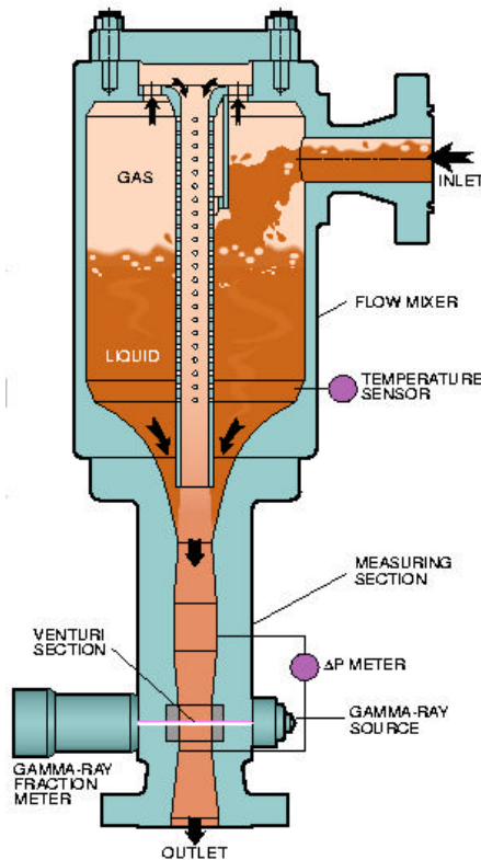
Figure 3: Example of a three-phase flowmeter which uses flow homogenization (courtesy of Framo Engineering AS)
