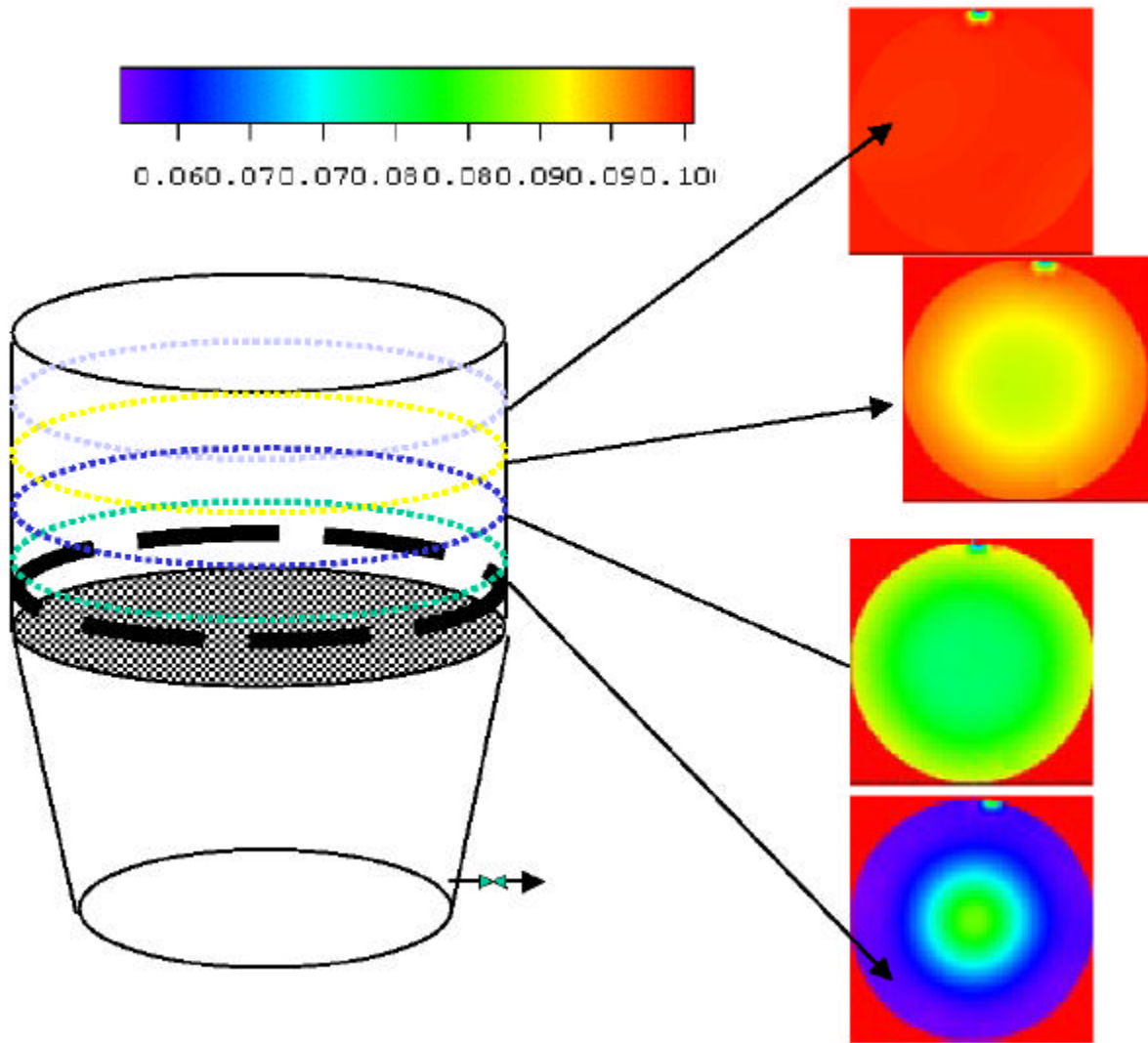
Figure 3 Mother liquor level detection during filtration using ERT
