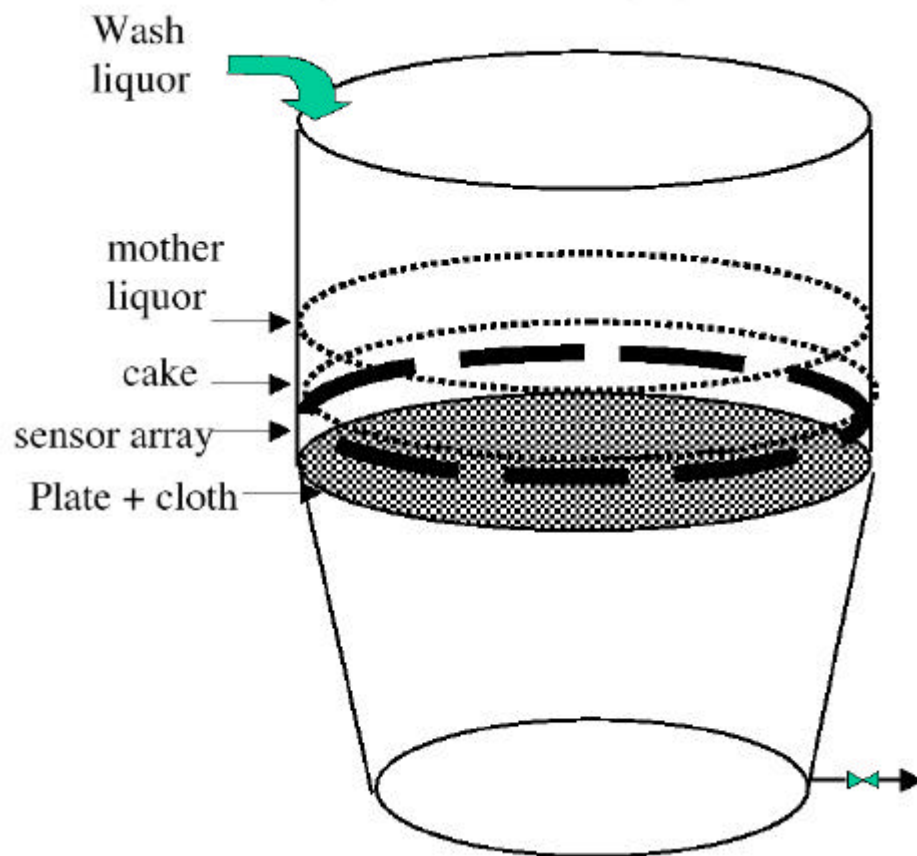
Figure 1 UMIST test filter
