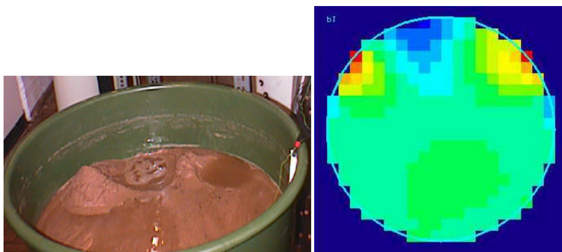
Figure 6 On-line detection of 2 large depressions in a sand filter cake
