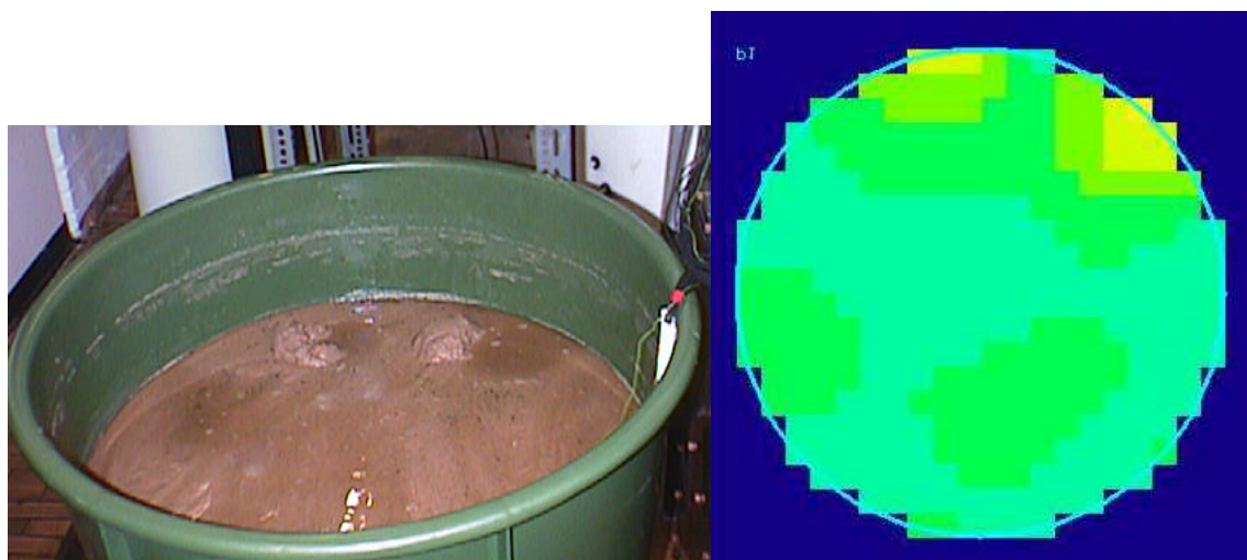
Figure 5 On-line detection of 2 shallow depressions in a sand filter cake
