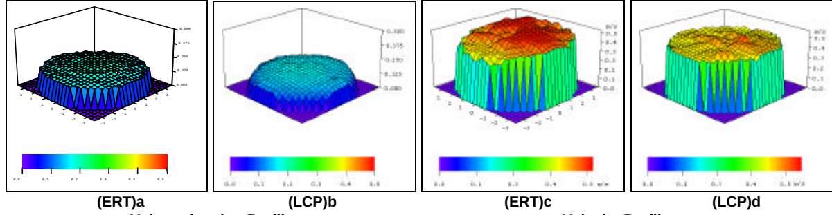
Figure 4 Volume Fraction and Velocity Profile Plots
