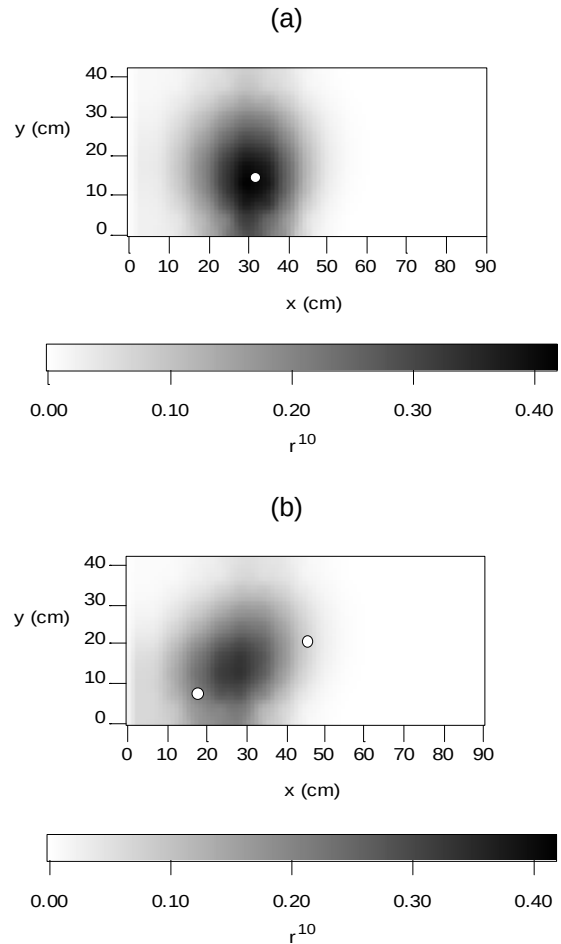
Figure 4: Example results of laboratory experiments showing correlation function plotted for two cases: (a) single leak, (b) dual leak. Circles indicate actual source location.
