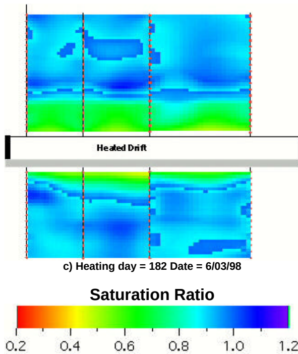
Figure 2: Maps of saturation change ratio from the 3 ERT planes above and the 3 planes below the heater drift. If the saturation does not change from baseline, the ratio would be 1.0 and if the saturation decreased it would be less than 1.0.
