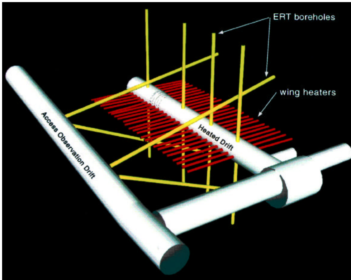
Figure 1: The Drift Scale Test layout in the Exploratory Studies Facility. A thermal bulkhead isolates the 47.5 m heated drift from the connecting drift and the access observation drift. The 12 boreholes used for ERT are also shown, 8 drilled from the heater drift and 4 drilled from the access observation drift.
