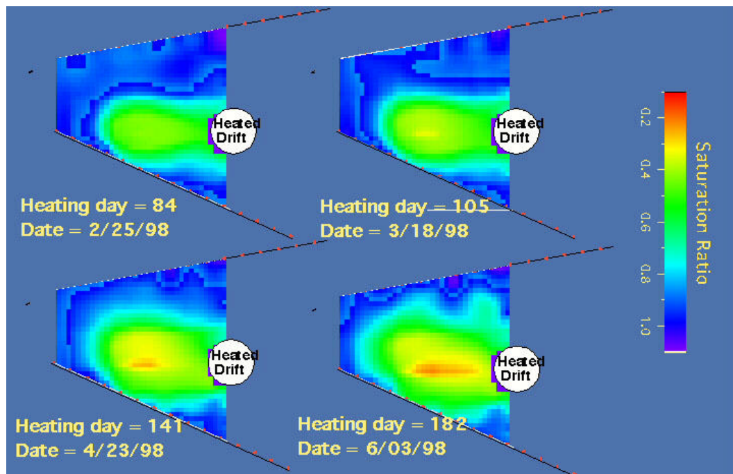
Figure 3: Maps of saturation change ratio from the 2 ERT planes perpendicular to the heater drift. The saturation scale is the same as for Figure 2.
